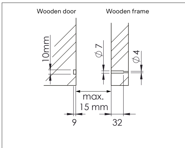
Figure 6.7-3. The embedding of the door switch and the magnet
