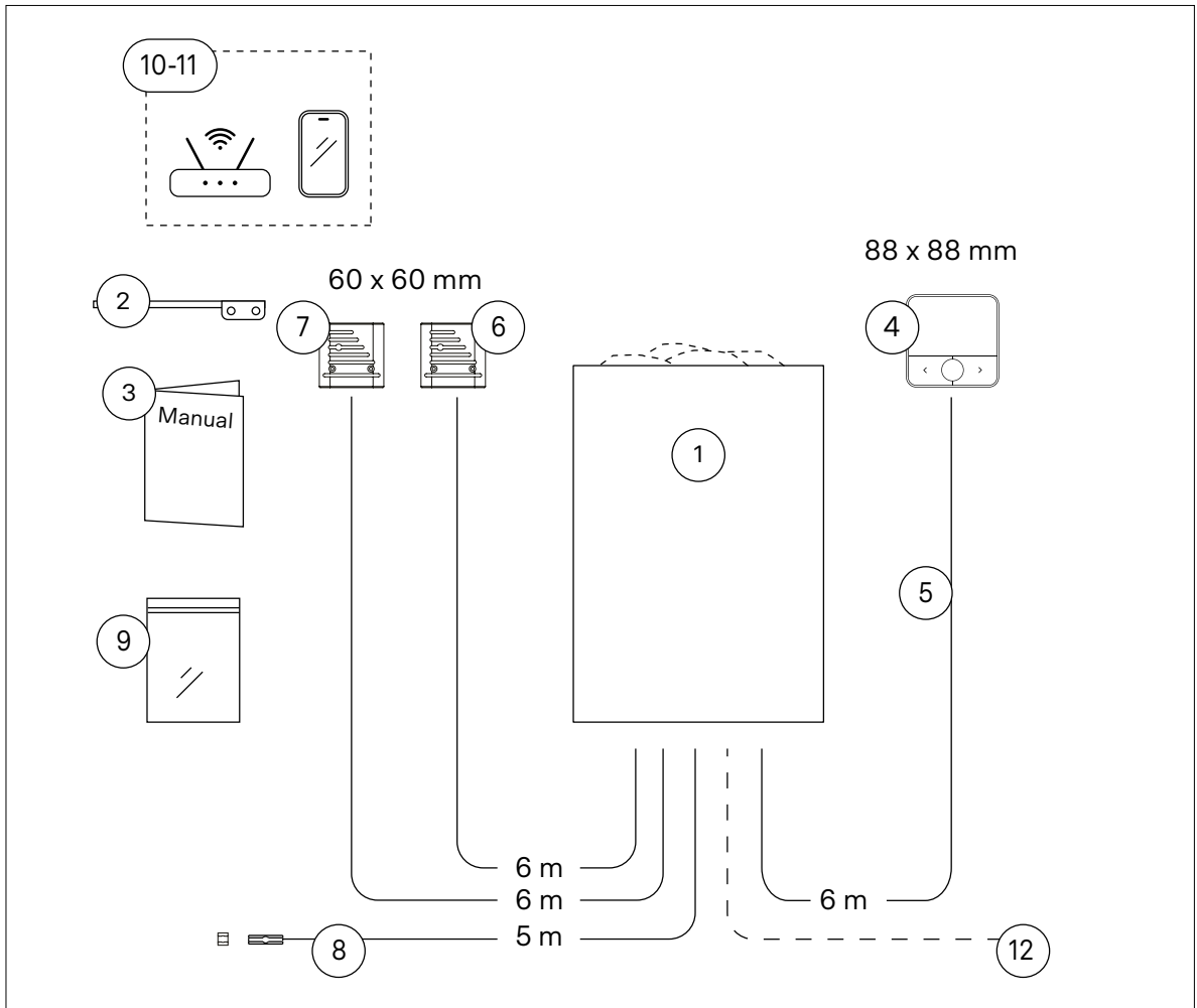
Figure 4.1-1 Bastusystemets delar
