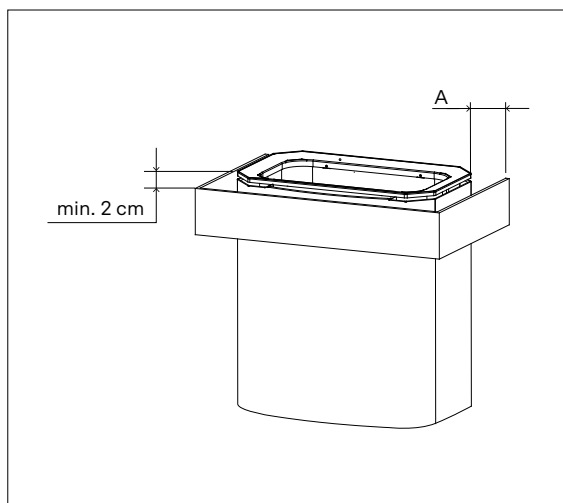
Figure 4.1-1. Heater guard
