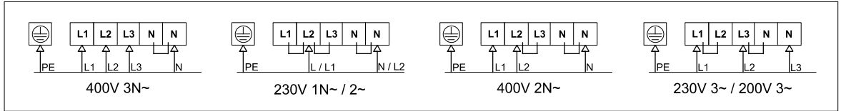
Figure 5.3-2. Connection diagram E-model / Flow with auxiliary power unit
