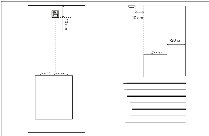
Figure 6.5-1. Installation of the temperature sensor
