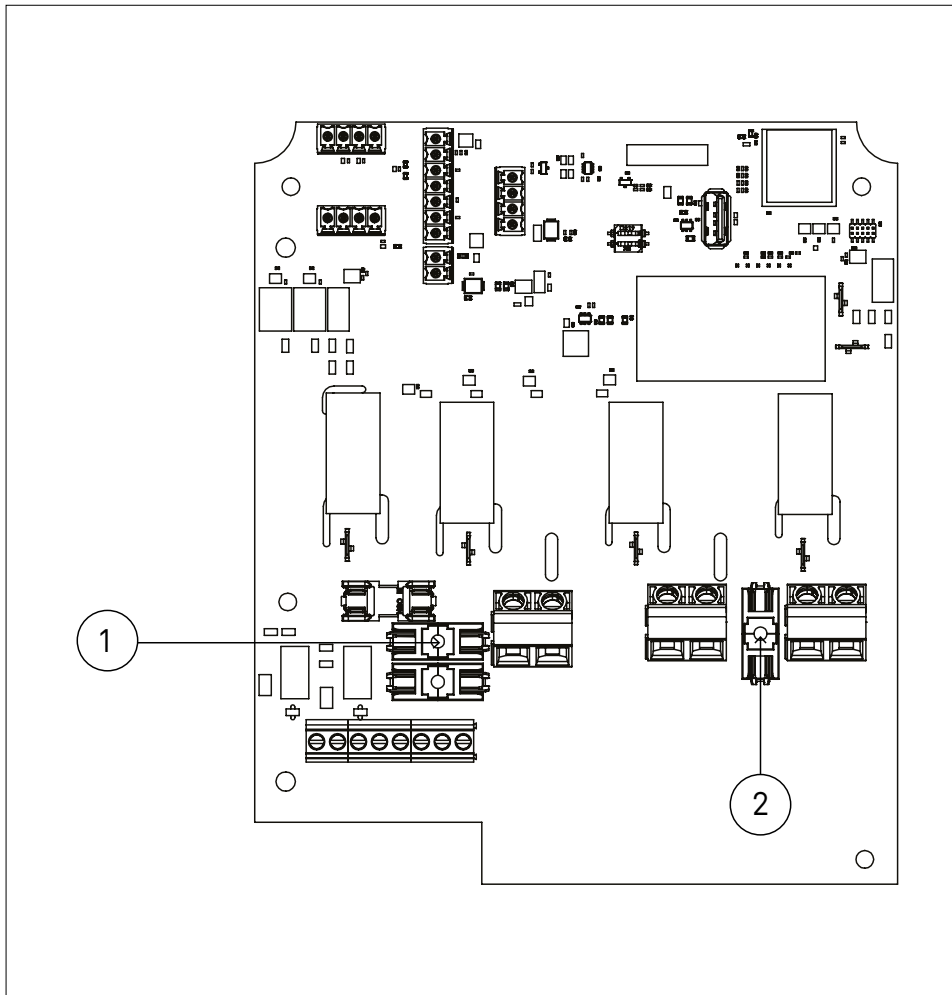
Figure 5.3-2. Circuit board fuses
