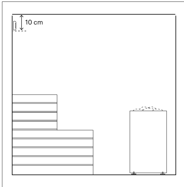
Figure 6.6.-1. Installation of the humidity sensor
